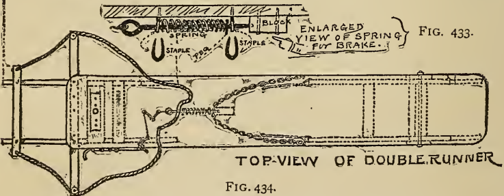
Working Plans for the Construction of Safety Double-Runner.
